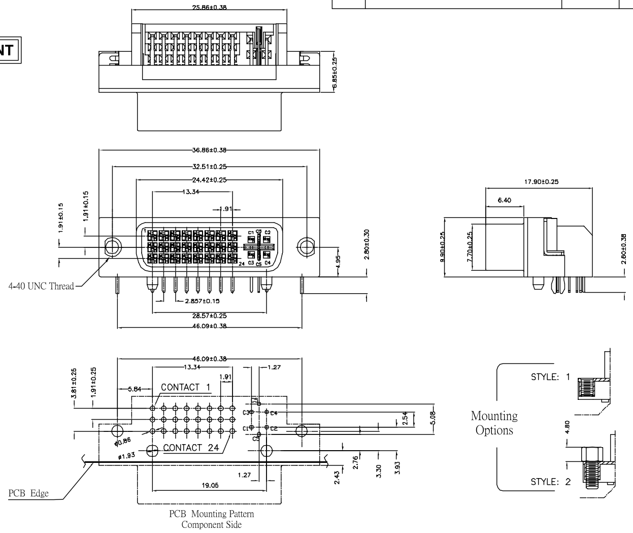
DVI CONNECTOR INTEGRATED 24+5 SOCKET RIGHT ANGLE TYPE
