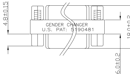
D-SUB 9.15.25.37 PIN (FEMALE)
