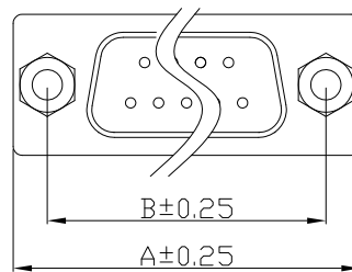
D-SUB 9.15.25.37 PIN (FEMALE)
