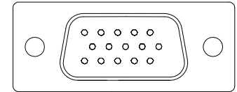
HD-15 PIN FEMALE
