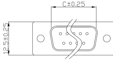
D-SUB 9.15.25.37 PIN (FEMALE)
